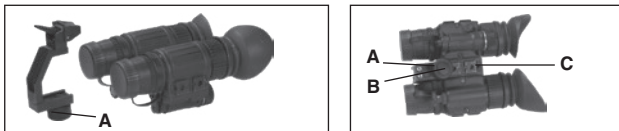
FIGURE 3-9. ATTACHING ADAPTER TO ATN PS-15
