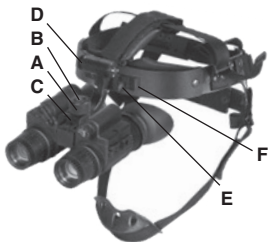
FIGURE 3-1. ATTACHING ATN PS-15 TO HEAD MOUNT
