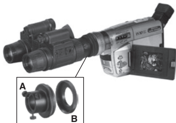
FIGURE 3-6. MOUNTING CAMCORDER TO THE ATN PS-15
